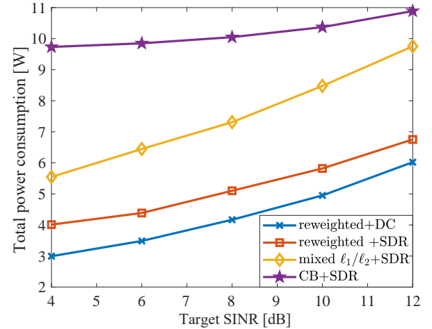
Fig. 8. Total power consumption over target SINR.
