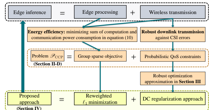
Fig. 1. Illustration of our energy-efficient processing and robust wireless cooperative transmission framework for edge inference.
