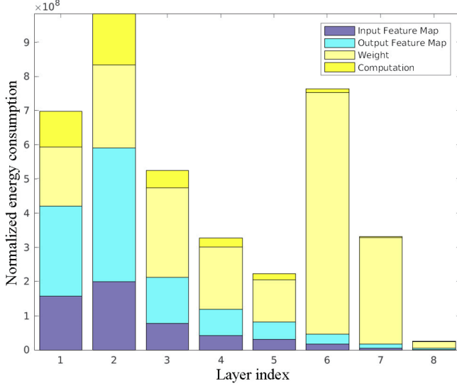
Fig. 3. Energy consumption breakdown of the AlexNet [28]. The unit of energy is normalized by the energy for one MAC operation (i.e., 10^2 = energy of 100 MACs).
